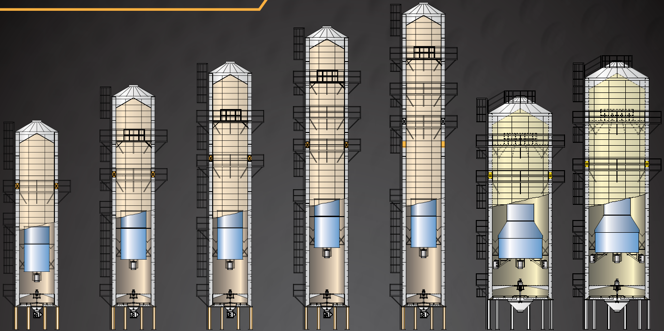
T-1575 12' dia. x 59'0" tall 19' dia. w/Catwalk
