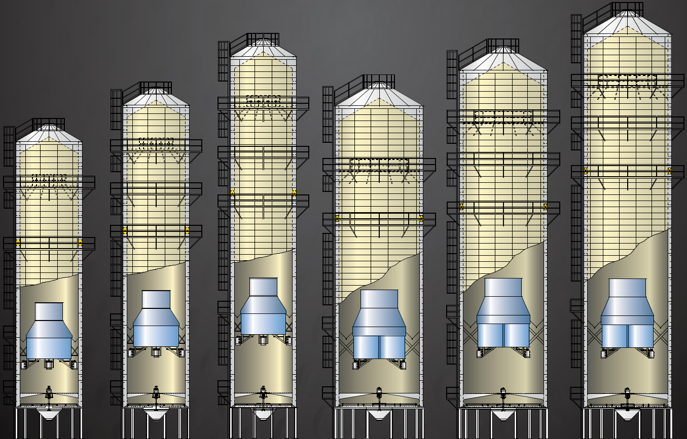
T-3531 18' dia. x 86'0" tall 25' dia. w/Catwalks
